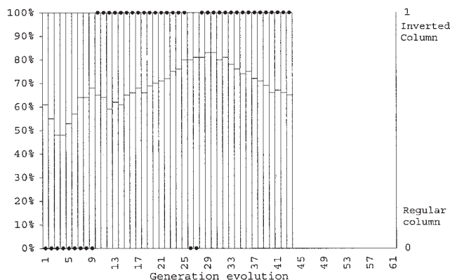
Figure 8. Percentage of column configurations in each generation of the genetic algorithm (feed 69.2 mol% cyclohexane).
