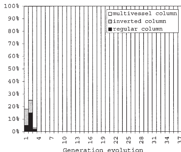
Figure 13. Percentage of column configurations in each generation of the genetic algorithm.
