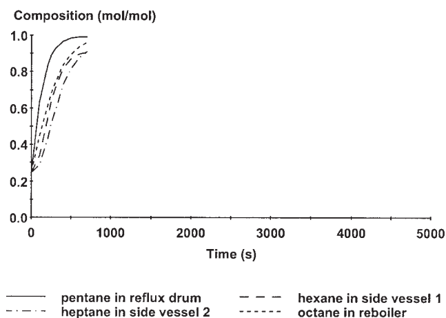
(c) Multivessel column
